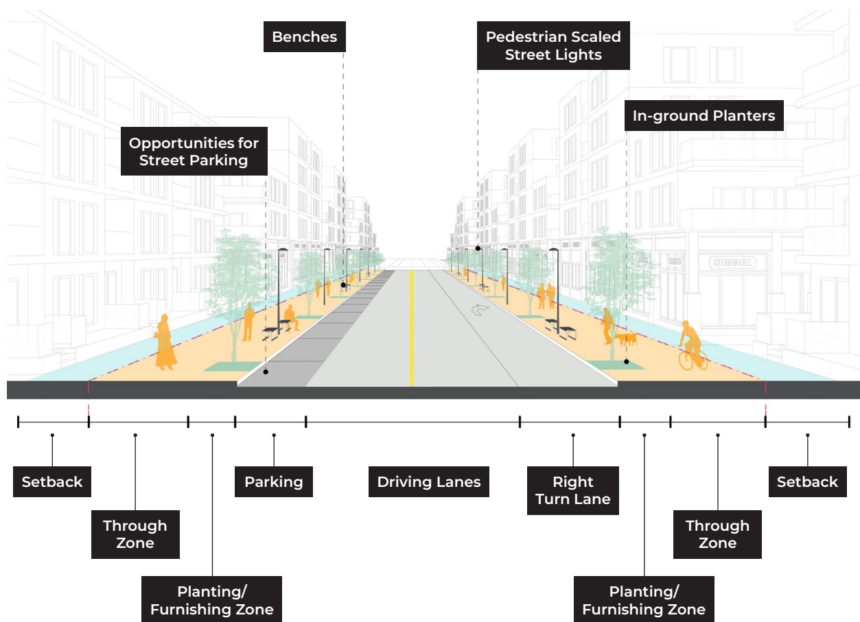
Figure 10: Collector Section
